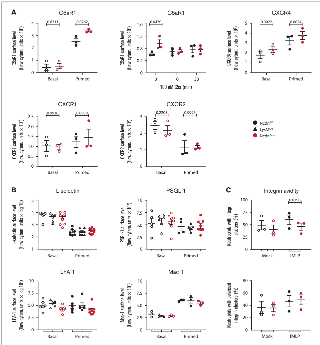
Figure 6. Norbin-deficient neutrophils have increased cell surface levels of the GPCRs C5aR1 and CXCR4 but normal surface levels of other receptors and adhesion molecules. (A) Ncdn fl/fl and Ncdn Δmye bone marrow cells were kept on ice (basal; open symbols) or were primed with 20 ng/mL TNF- \alpha , 50 ng/mL GM-CSF for 45 minutes at 37°C before transfer onto ice (filled symbols). Cells were stained to identify neutrophils and quantify the mean levels of C5aR1, CXCR4, CXCR1, and CXCR2 on the neutrophil surface by flow cytometry. (Top, middle panel) Bone marrow cells were incubated for 30 minutes at 37°C without or with 100 nM C5a, or C5a was added for the last 10 minutes as indicated, before transfer onto ice and quantification of the mean C5aR1 level on the neutrophil surface. Data are mean \pm standard error of the mean (SEM) of 3 independent experiments; each dot is the mean of 1 experiment. (B) Ncdn fl/fl , LysM Cre , and Ncdn Δmye bone marrow cells were treated as in panel A and stained to identify neutrophils and quantify the mean levels of L-selectin, PSGL-1, LFA-1, and Mac-1 on the neutrophil surface by flow cytometry. Data are mean \pm SEM of 3 to 8 independent experiments; each dot is the mean of 1 experiment. (C) Integrin avidity. Purified Ncdn fl/fl and Ncdn Δmye neutrophils were primed with 20 ng/mL TNF- \alpha , 50 ng/mL GM-CSF for 45 minutes at 37°C before incubation with AF594-labeled anti-CD18 antibody for 3 minutes at 37°C in the presence (filled symbols) or absence (open symbols) of 1.5 \mu M fMLP. Cells were fixed and allowed to settle onto electrostatically charged slides before imaging and image analysis for the presence and localization of integrin clusters. A total of 30 to 40 cells were analyzed/condition/experiment. Data are mean \pm SEM of 3 independent experiments; each dot represents 1 experiment. Statistics in panels A to C comprised two-way analysis of variance with Sidák's multiple comparisons test.
